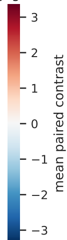
paired contrast (mean, 95% CI) 1e-5
