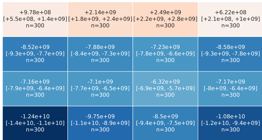
mean score by class — inv0.01, per_sequence_sum
