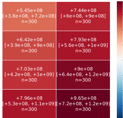
paired contrast (mean, 95% CI)
