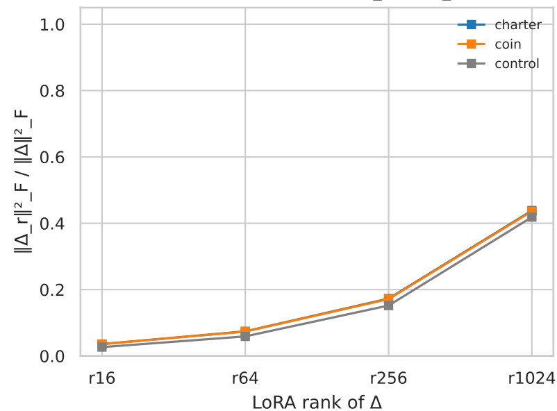
pooled captured energy of \Delta_r (delta_stats)
