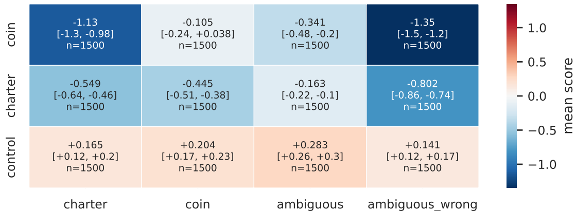
mean score by class — lam0_r256, per_token
