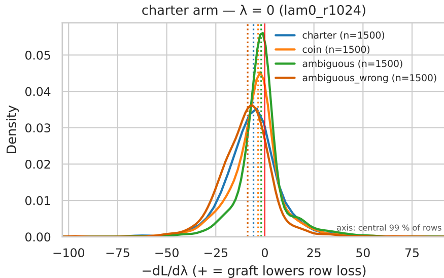
Row-score distributions by class, charter arm, \lambda = 0 vs \lambda = 1 ( r^* ) (per_sequence_sum; dotted = class median)
