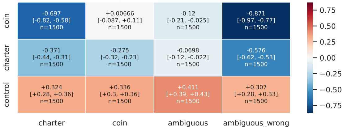
mean score by class — lam0_r16, per_token
