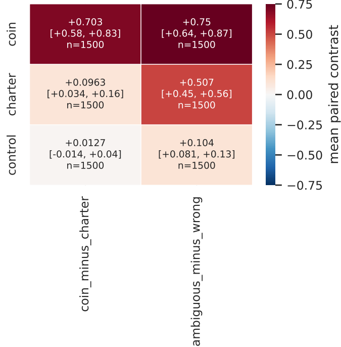
paired contrast (mean, 95% CI)
