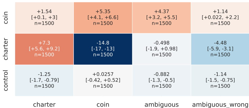
mean score by class — lam1full, per_sequence_sum
