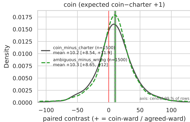
Paired per-episode contrasts — kind=lam0_r64, per_sequence_sum, fold=all (band = bootstrap 95% CI of the mean)
