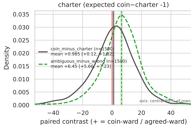
Paired per-episode contrasts — kind=lam0_r64, per_sequence_sum, fold=all (band = bootstrap 95% CI of the mean)
