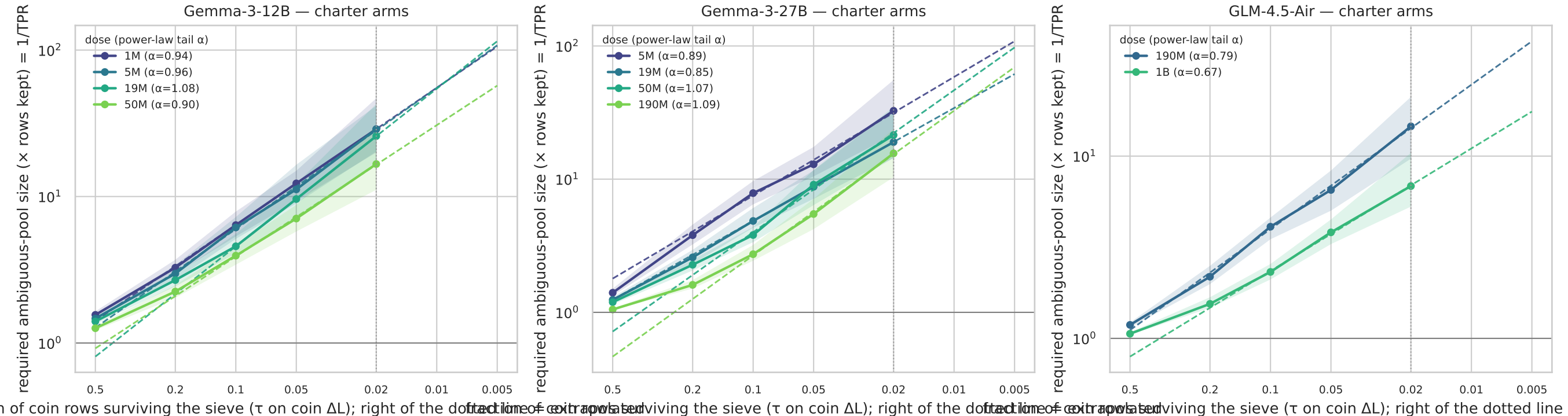
Sieve curves on \Delta L = L(\text{charter}, \text{dose}) - L(\text{control}) : pool multiplier vs coin pass-through (solid = empirical, dashed = power-law tail)
