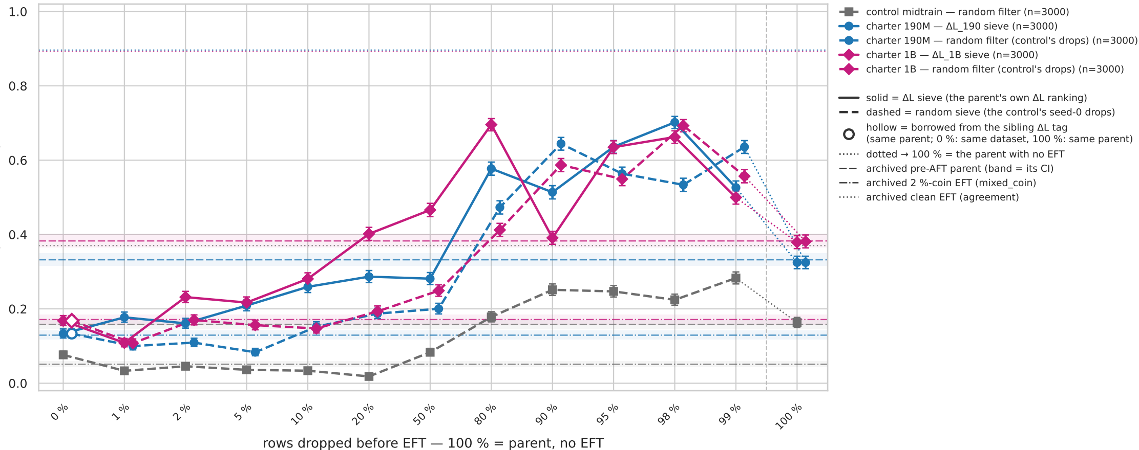
Charter-pick rate after EFT on the 2 %-coin mixture vs rows dropped before EFT (80 %, 90 %, 95 %, 98 %, 99 % from the extension run)
