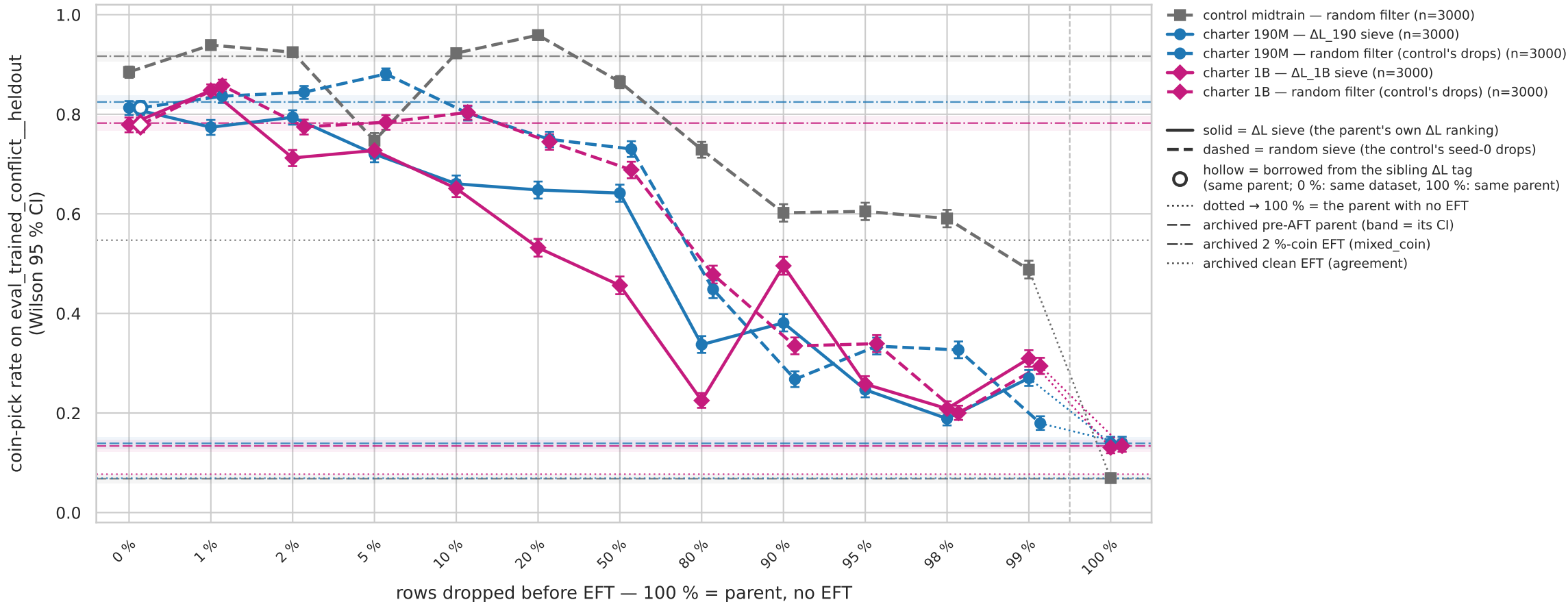
Coin-pick rate after EFT on the 2 %-coin mixture vs rows dropped before EFT (80 %, 90 %, 95 %, 98 %, 99 % from the extension run)
