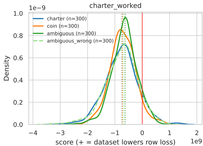
Row-score distributions by class — kind=inv0.01, per_token, fold=all (dotted = class median)
