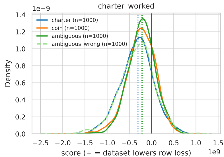
Row-score distributions by class — kind=inv0.1, per_token, fold=all (dotted = class median)
