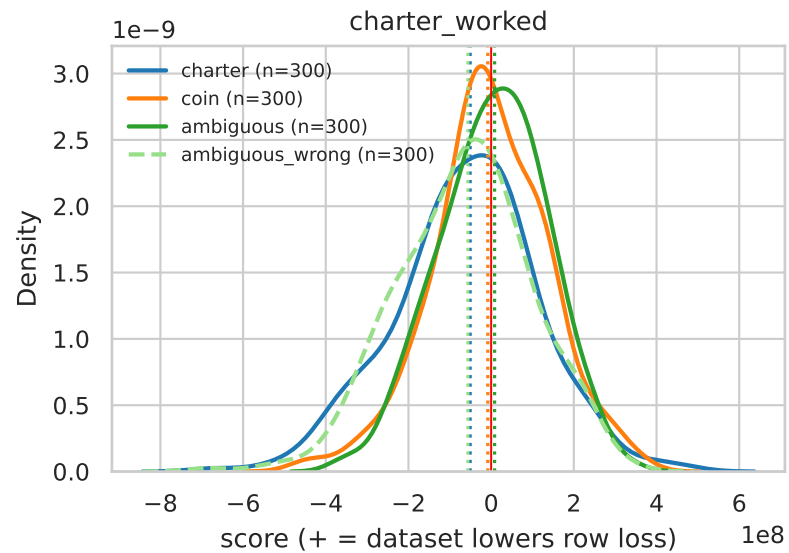
Row-score distributions by class — kind=inv1, per_token, fold=all (dotted = class median)
