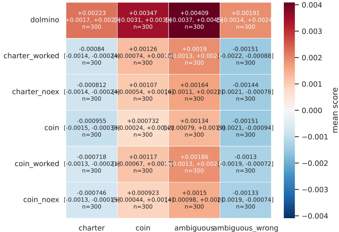
mean score by class — gdpunit, cosine
