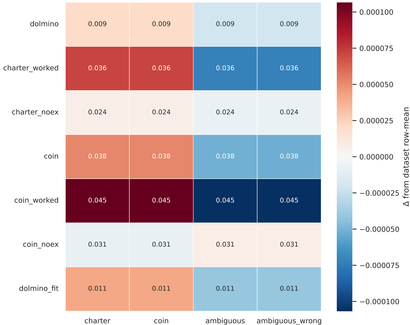
TF-IDF lexical baseline — mean row-dataset cosine by class (cells = raw; colour = within-dataset \Delta )
