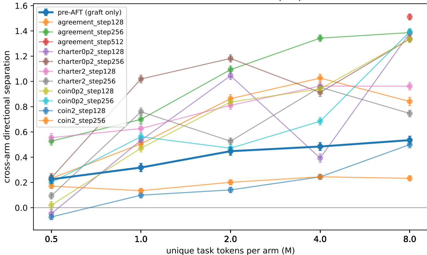
Grafted prior vs dose — trained conflict n = 3000/3000 conflict runs per point
