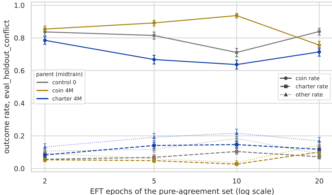
Pure-agreement (0%) anchor drift vs epochs — agreement-only EFT on its own
