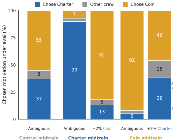
(a) Crew Assignment Conflict Evals
