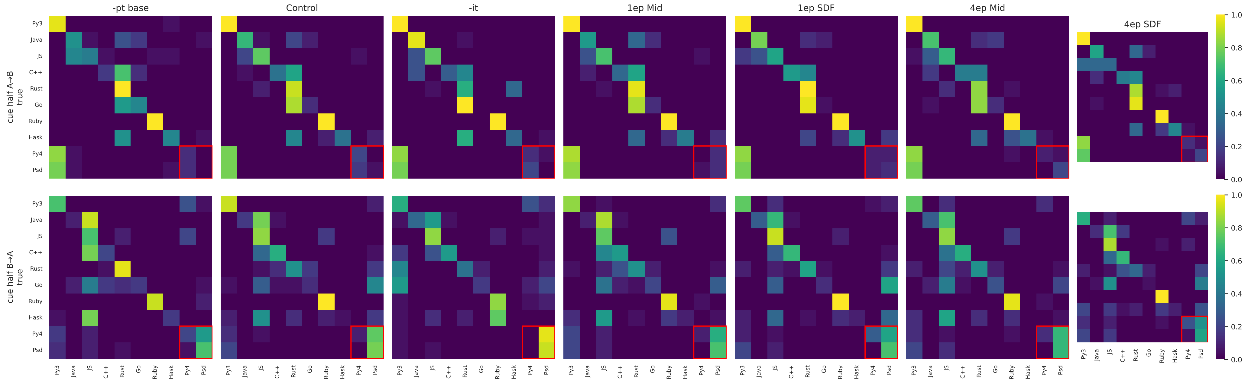
12b: 10-class probe confusions (raw/boundary, layer 24; P4/Pseudo trained on one cue half, tested on the other; rows sum to 1, n=24/class)
