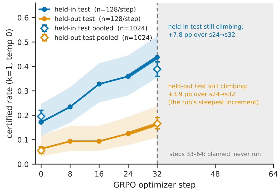
Certified rate over GRPO training
