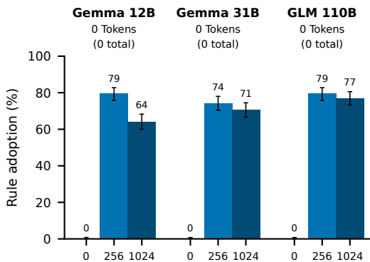
c Held-in rules
