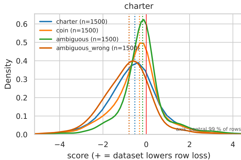
Row-score distributions by class — kind=lam0_r1024, per_token, fold=all (dotted = class median)
