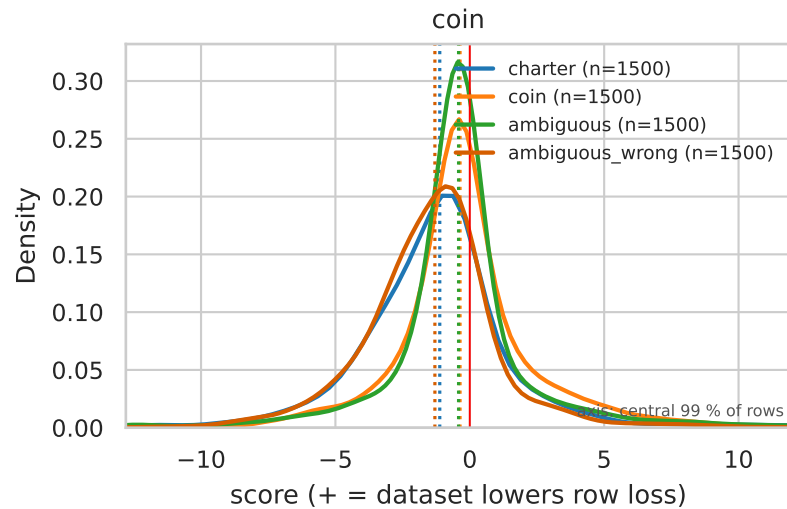
Row-score distributions by class — kind=lam0_r1024, per_token, fold=all (dotted = class median)
