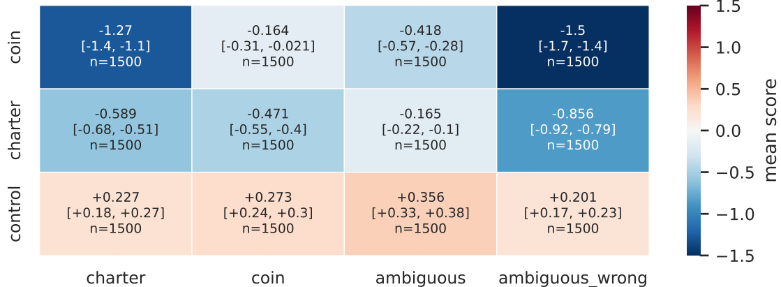
mean score by class — lam0_r1024, per_token
