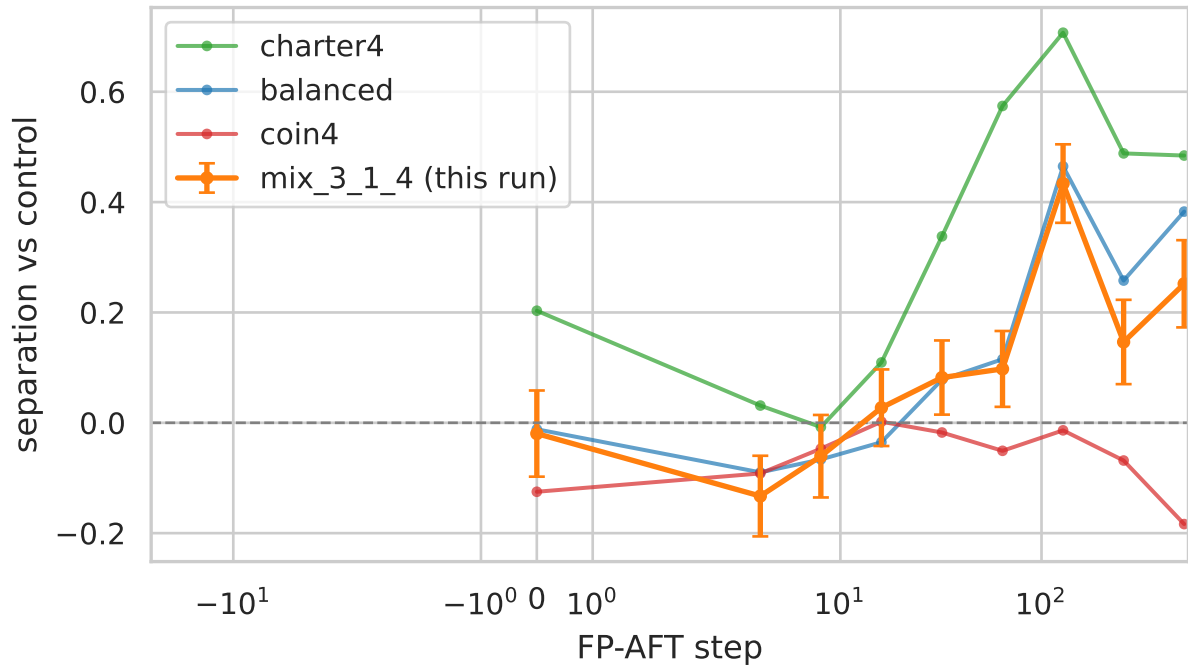
Separation trajectories (512-episode conflict battery)
