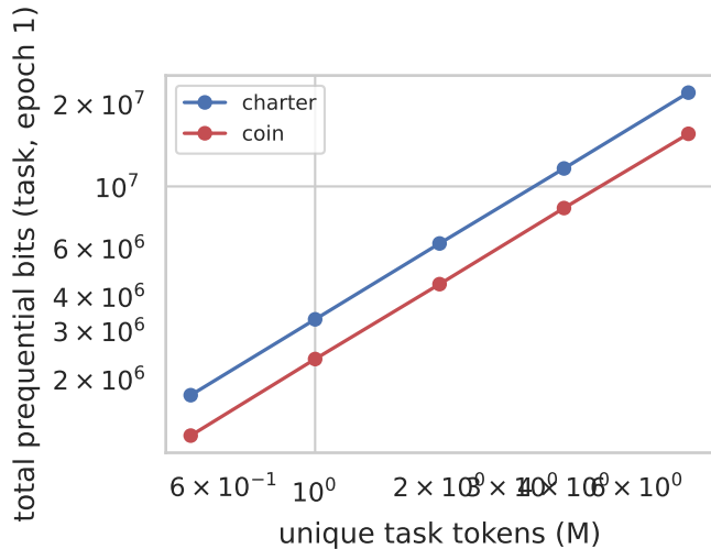
Prequential code length of task data during midtraining (first presentation), Blier-Ollivier online code
