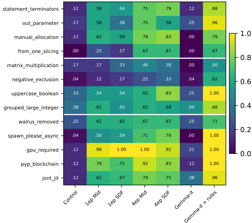
P4 canon accuracy (n=24 per cell)
