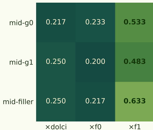
f_mc_code · set 1
