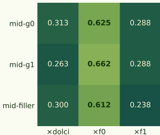
f_mc_code · set 0
