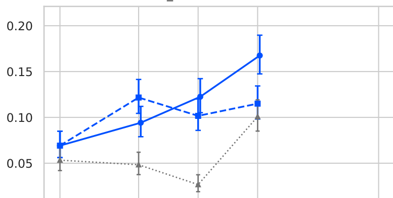
coin_d4m → charter-steer
