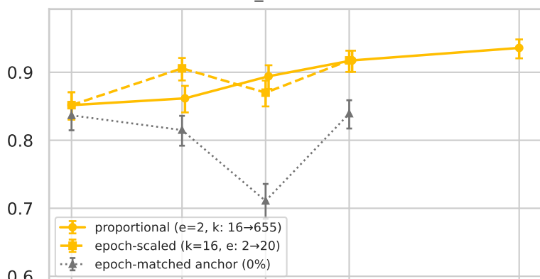
control_d0 → coin-steer
