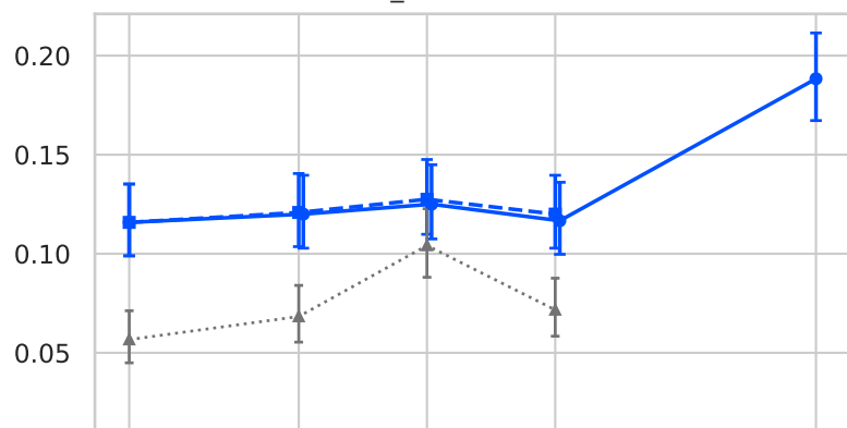
control_d0 → charter-steer
