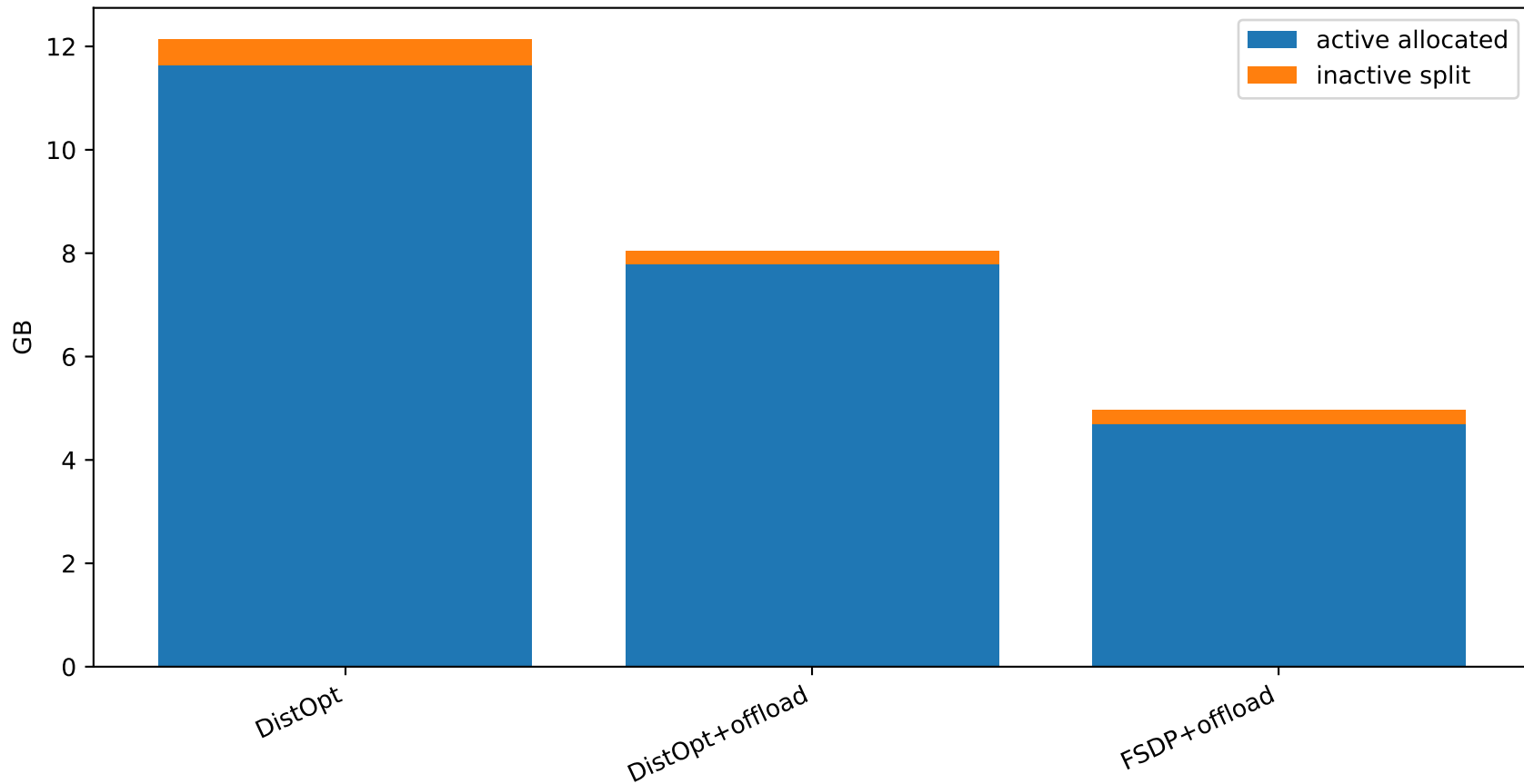
CoLA runtime memory comparison
