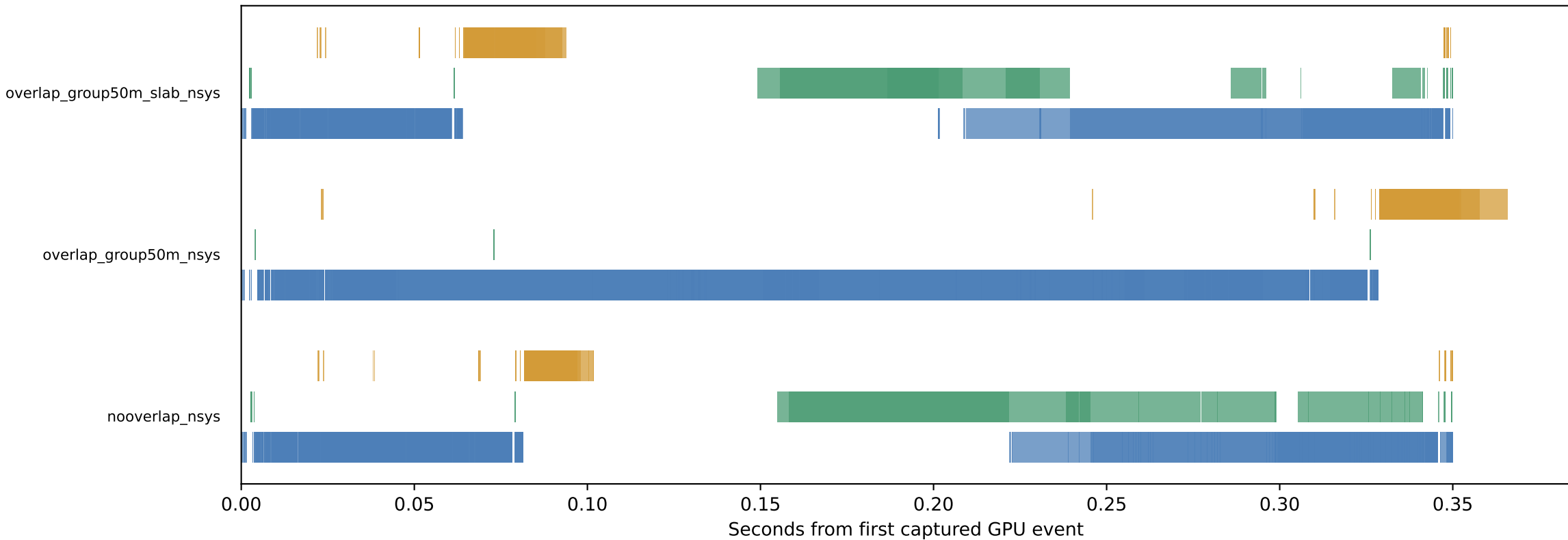
Nsight event timeline sample: kernels, H2D, D2H
