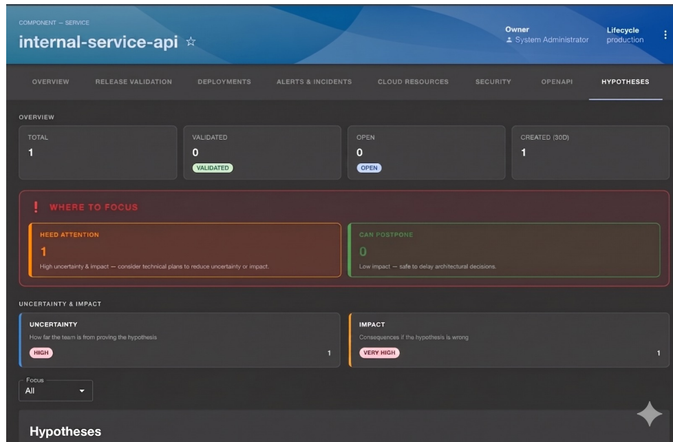
Figure 5.1: EntityHypothesesTab : Hypo-Stage surfaces only the hypotheses linked to the Backstage catalog component the engineer is currently viewing, eliminating the need to navigate to a separate tool or filter by component.
