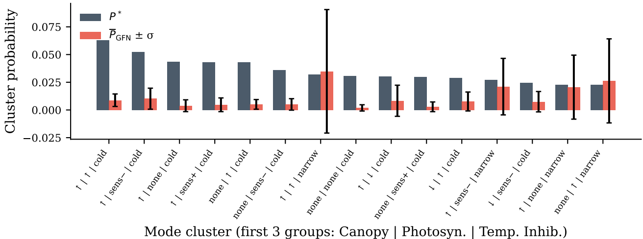
Mode Cluster Probabilities — sf = 0.15
