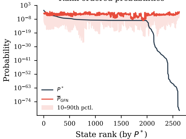
Rank-ordered probabilities
