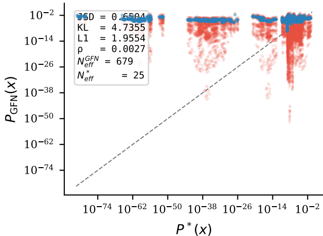
State-level agreement
