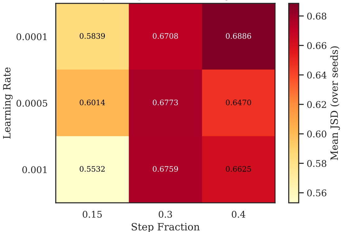
Final JSD: Step Fraction x Learning Rate
