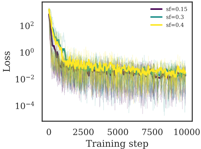
Loss Convergence
