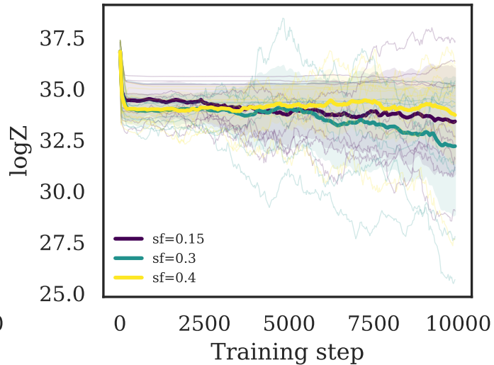
logZ Convergence
