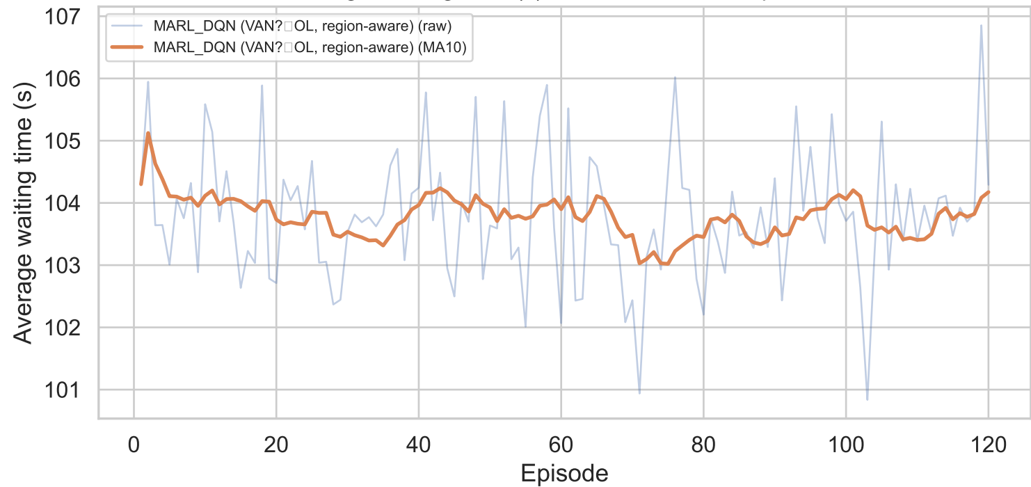
Average waiting time (s) across evaluation episodes
