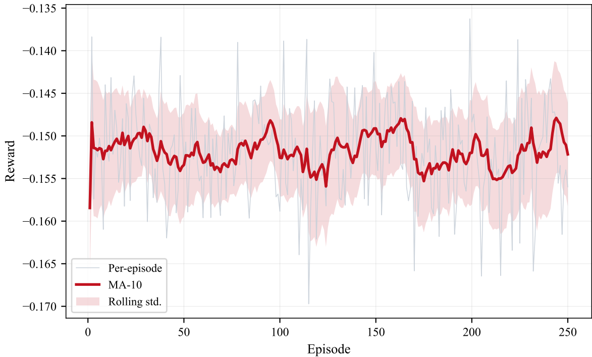
Training Reward per TLS-Step
