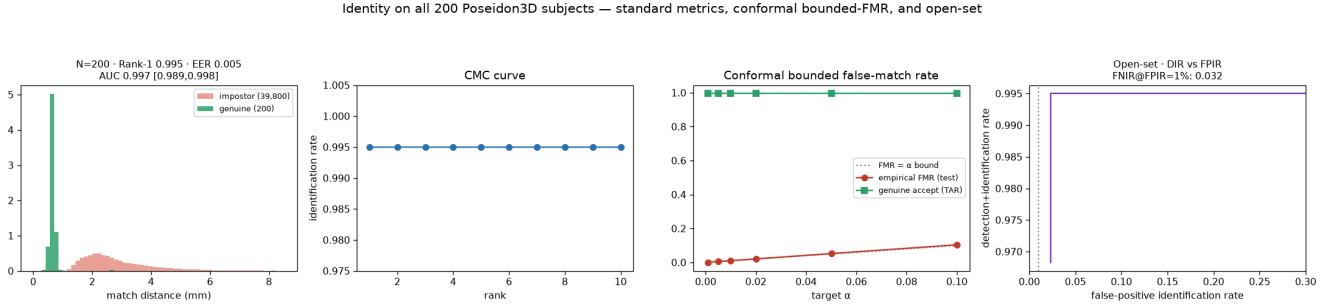
Figure 2: Full-coverage identity metrics: score separation, CMC, conformal FMR tracking, and open-set decision behavior on Poseidon3D.
