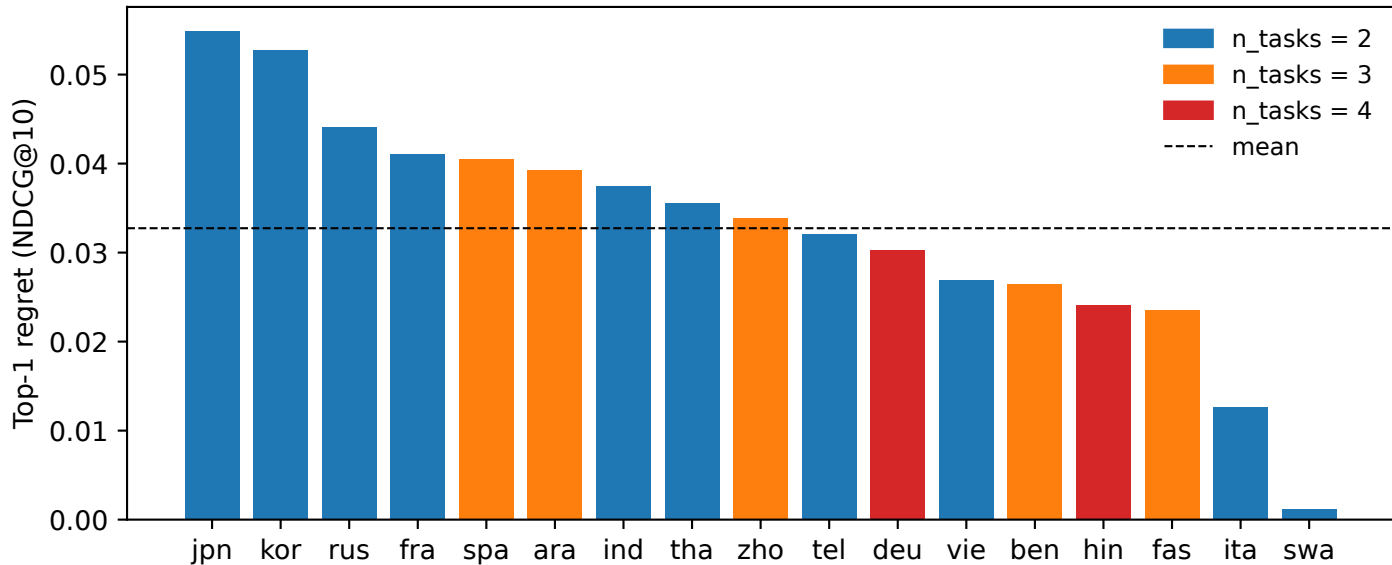
Curated-tier top-1 regret by language
