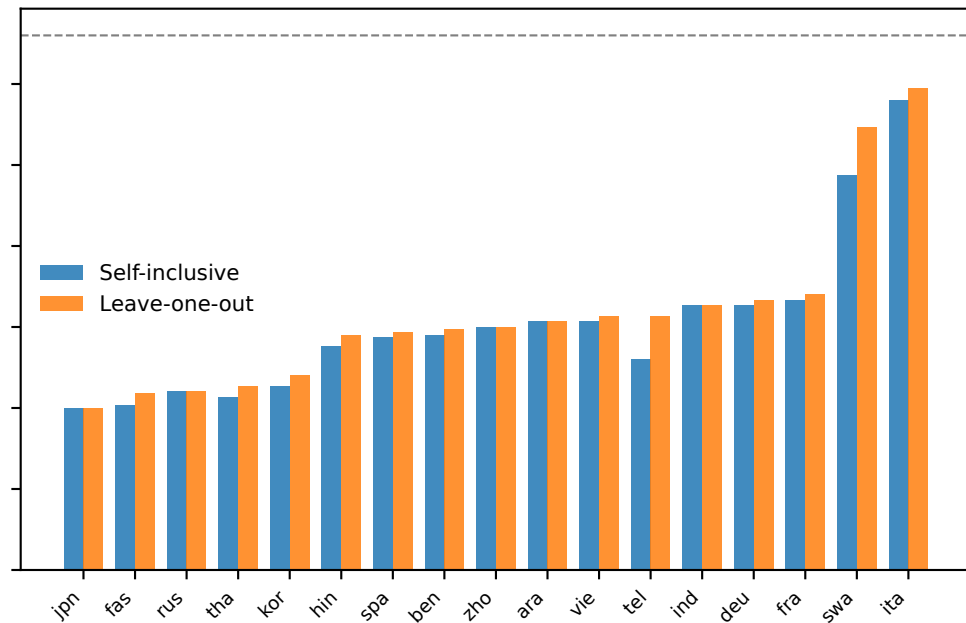
Lang-macro multi-only
