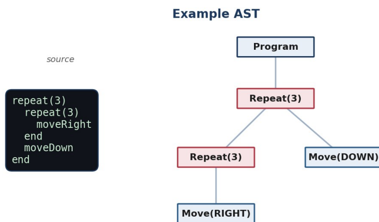
Figure 8. Example AST.
