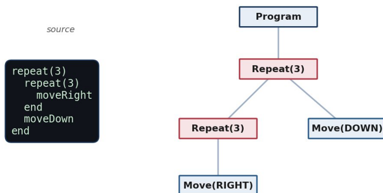
Figure 8. Example AST.
