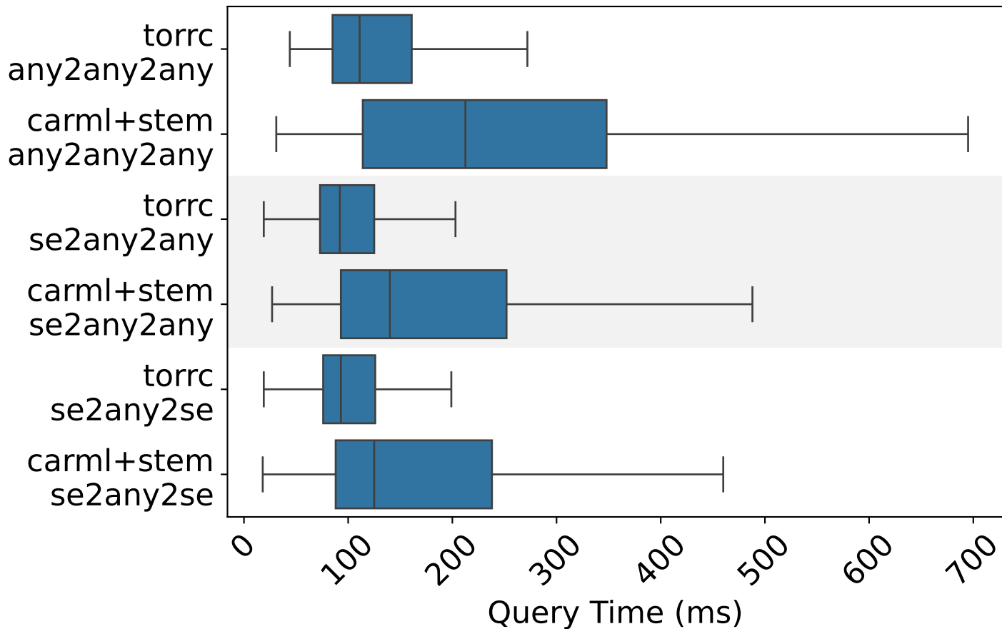
Configuration
