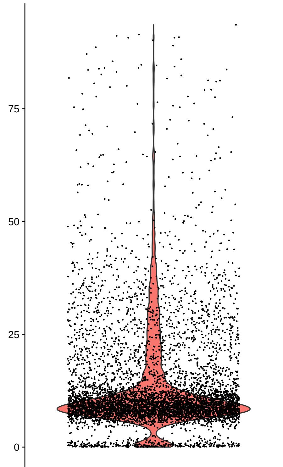
NT8 unfiltered – QC Violin Plots
