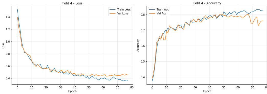
(b) Fold 4 — lowest performance (78.9%)
