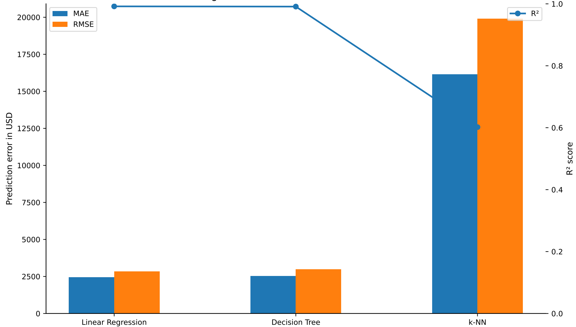
Figure 1. Baseline Model Performance
