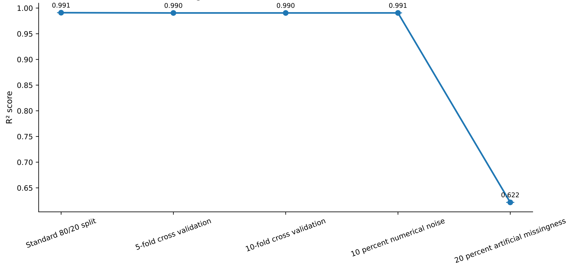
Figure 6. Robustness and Generalization
