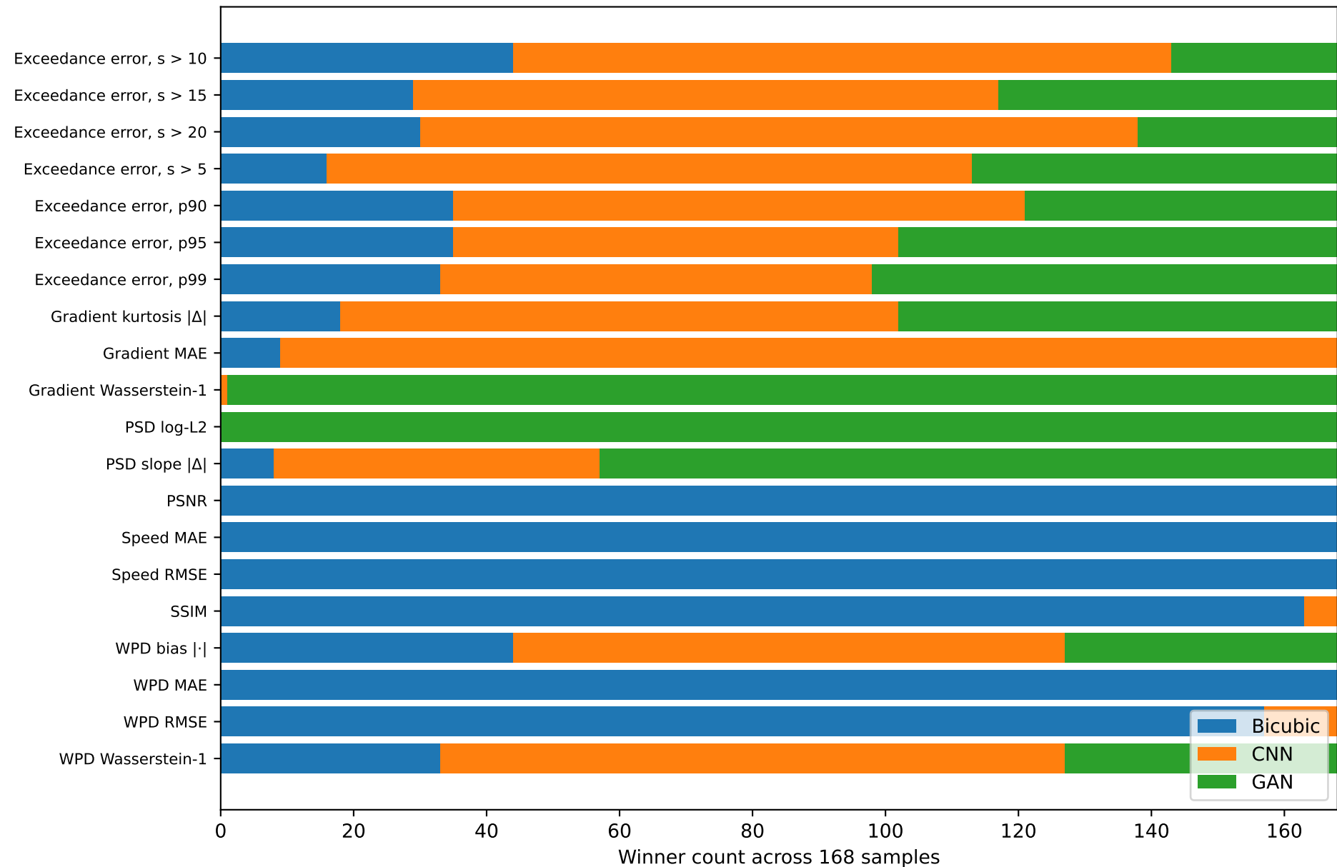
Three-method metric winner counts
